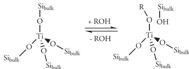
Scheme 2. Addition of water or TBHP to an isolated, tetrahedral Ti site yielding a tripodal Ti site and a neighboring SiOH (R = H or t\text{BuO} ).
